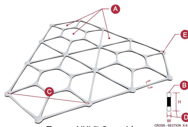
Tensar NXL™ Geogrid Plan View
