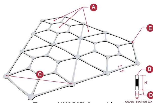
Tensar NX850™ Geogrid Plan View
